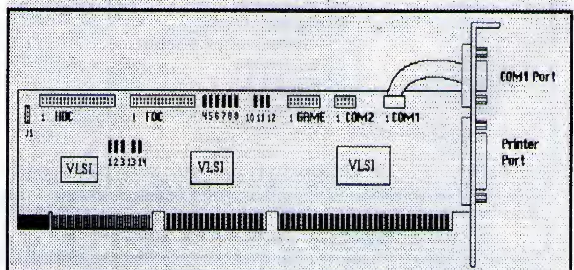
Figura 15 - placa IDEPLUS VLB (32 bits)
